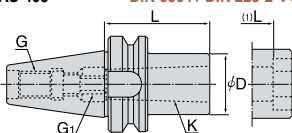
BT MAS-403
