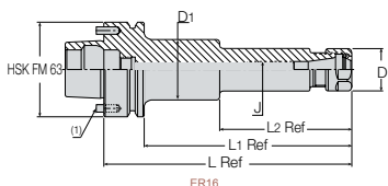
DIN69896 FM (1)
