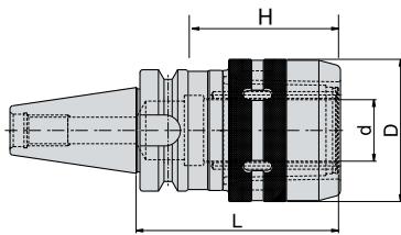
BT MAS-403
